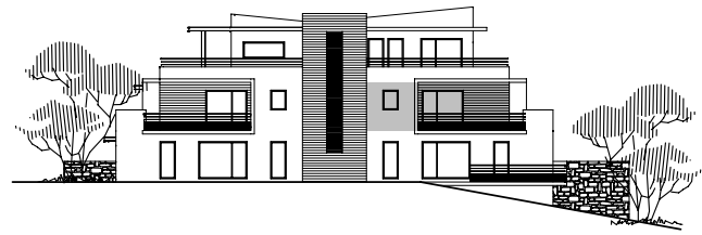
FACADE ARRIERE
